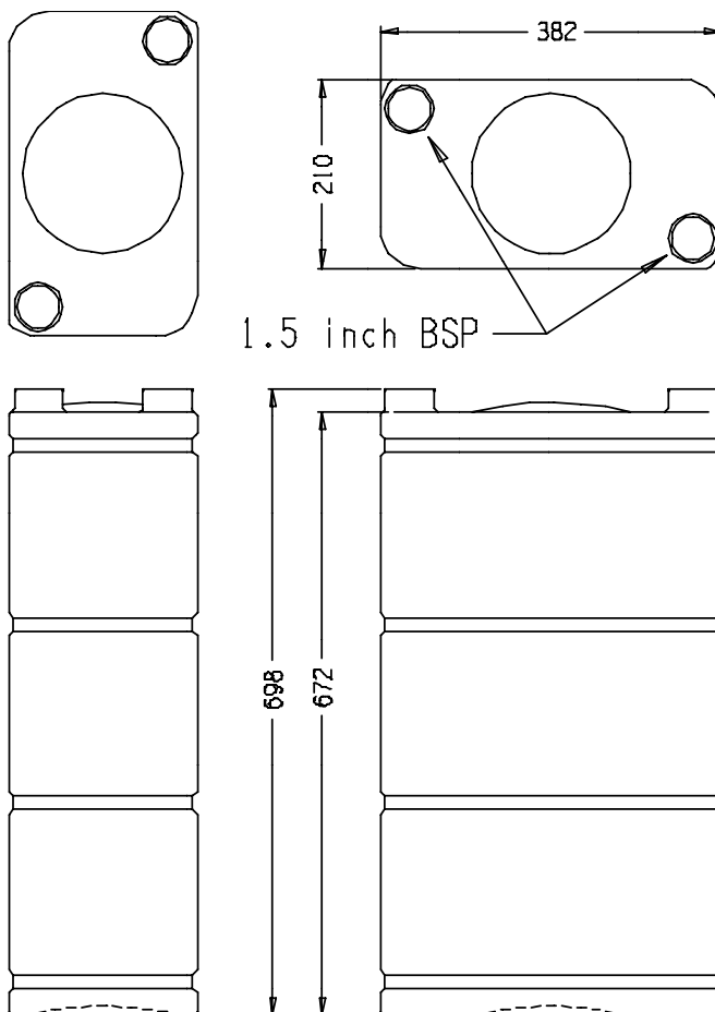
Single Tank Dimensions 50 Litre Tank Part No 200003 Weight 2.5Kg
